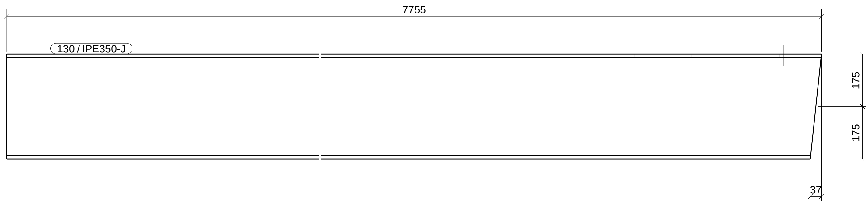
FRONT VIEW
